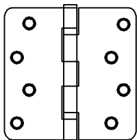
1/4" radius corner 4.0" x 4.0" pictured
