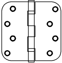
5/8" radius corner 4.0" x 4.0" pictured
