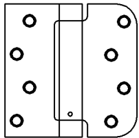
square corner x 5/8" radius 4.0" x 4.0" pictured
