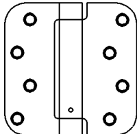
5/8" radius corner 4.0" x 4.0" pictured
