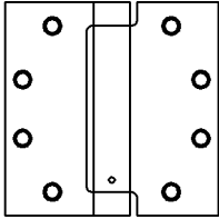
square corner 4.5" x 4.5" pictured
