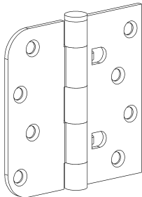
5/8" radius x square corner
